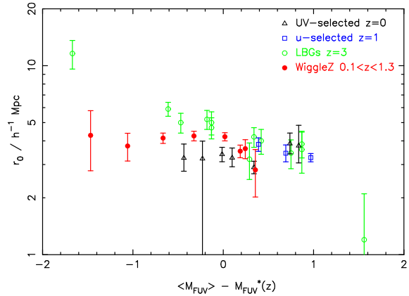
Figure 16. Comparison of the clustering segregation with FUV absolute magnitude observed in the WiggleZ sample with the compilation of low-redshift and high-redshift results presented by Heinis et al. (2007). The WiggleZ targets are more comparable to z = 3 LBGs rather than z = 0 UV-selected galaxies. The displayed data points are obtained from Giallisco & Dickinson (2001), Arnouts et al. (2002), Foucaud et al. (2003), Heinis et al. (2004), Adelberger et al. (2005) and Heinis et al. (2007). Absolute magnitudes are calculated assuming h = 0.7 .
